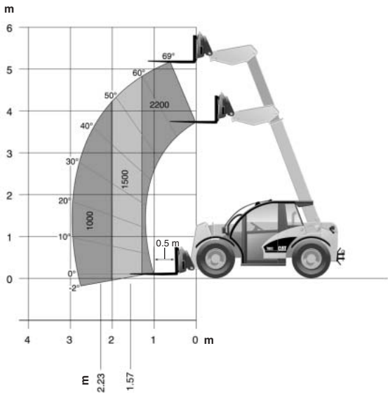
TH210 Non-U.S. Version
