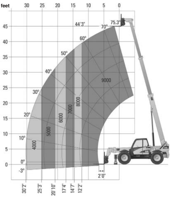
TH460B Stabilizers Down
