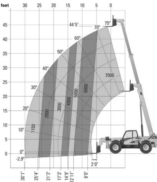
TH360B Stabilizers Up
