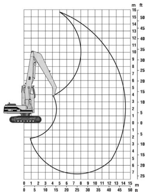
330C MH Range Diagram
