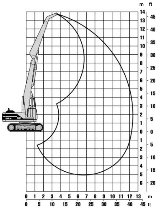
320C MH Range Diagram
