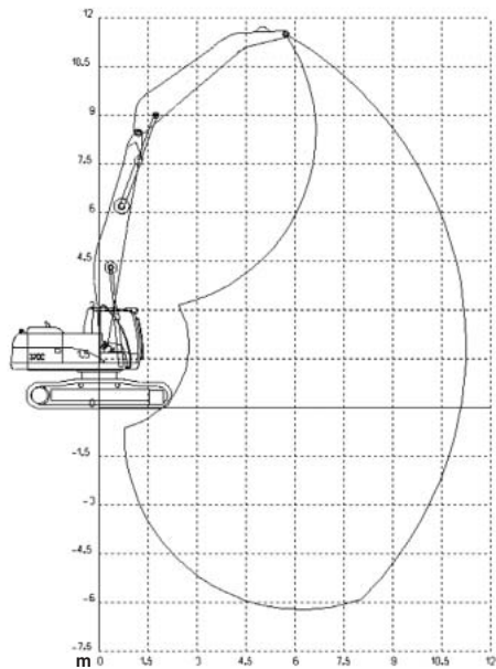
330C MH Range Diagram — U.S. Sourced ● Caterpillar Material Handling Boom and Stick
