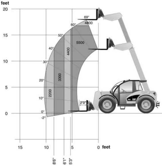
TH215 North American Version
