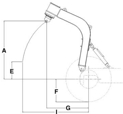
Single Function Frame Group
