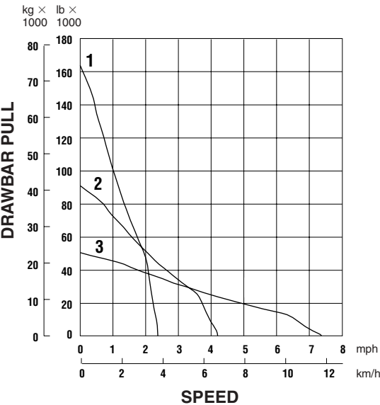
D9R Differential Steering
