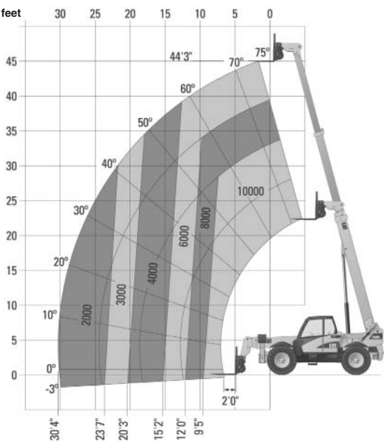
TH560B Stabilizers Up
