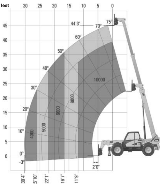
TH560B Stabilizers Down
