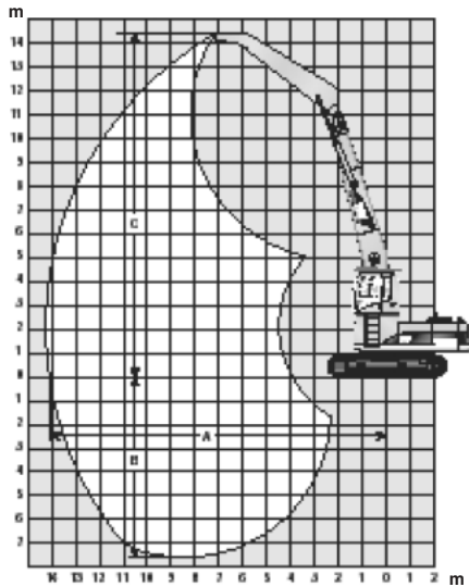
320C L MH, 325C L MH, 330C L MH, 345B L Series II MH, 365B L Series II MH Range Diagram
