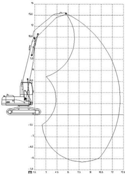
325C MH Range Diagram — U.S. Sourced ● Caterpillar Material Handling Boom and Stick
