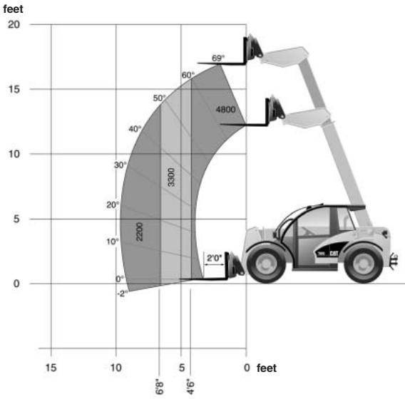
TH210 North American Version
