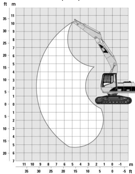
6.18 m (20'2") Mass Boom with 3.52 m (11'6") Reach Stick
