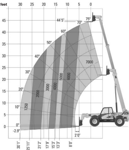
TH360B No Stabilizers
