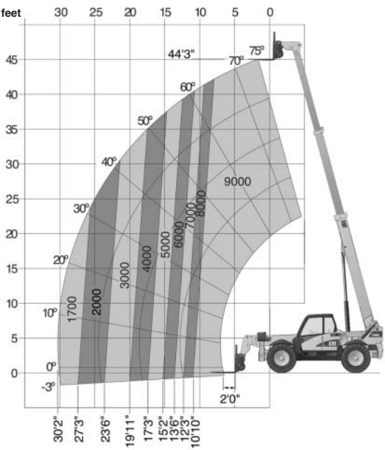
TH460B Stabilizers Up
