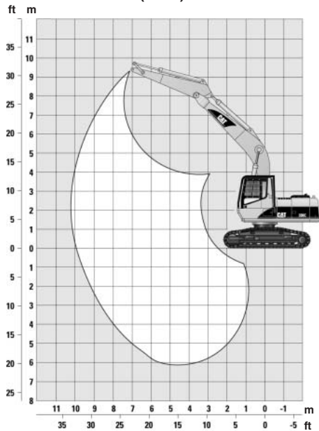
6.5 m (21'2") Reach Boom with 3.9 m (12'9") Reach Stick
