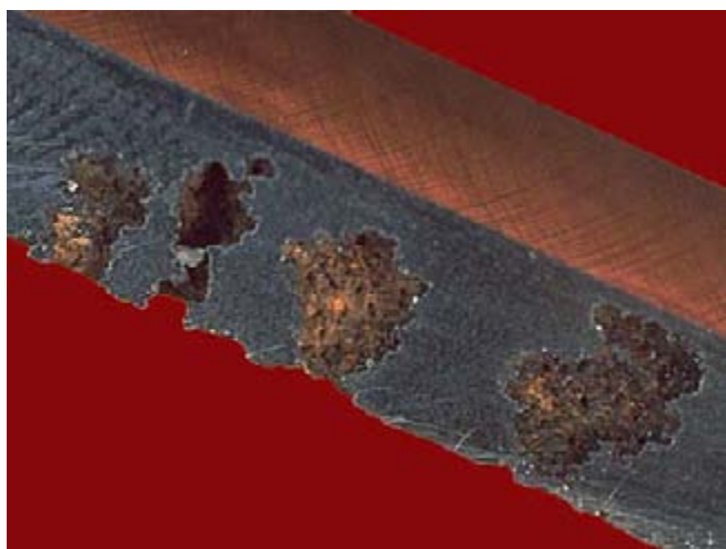
Fig. 41: Careful examination of what appears to be small surface pits in Fig. 37 will reveal large underlying holes in the liner wall. This is called concentration cell pitting corrosion.
