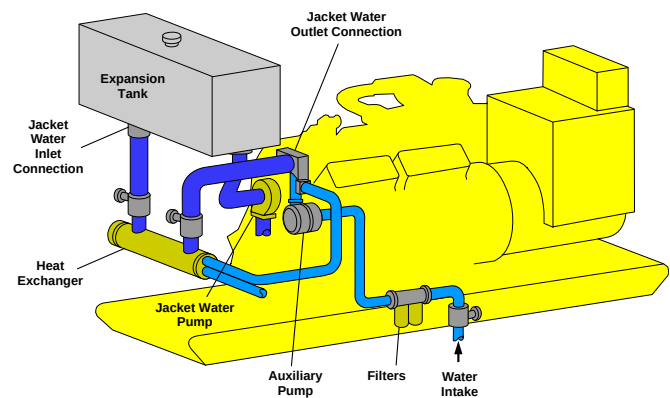
Fig. 3: Schematic of typical heat exchanger cooling system.
