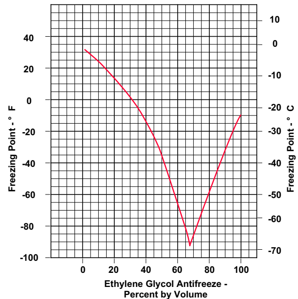
Fig. 17: Freezing point curve for typical ethylene glycol solution.
