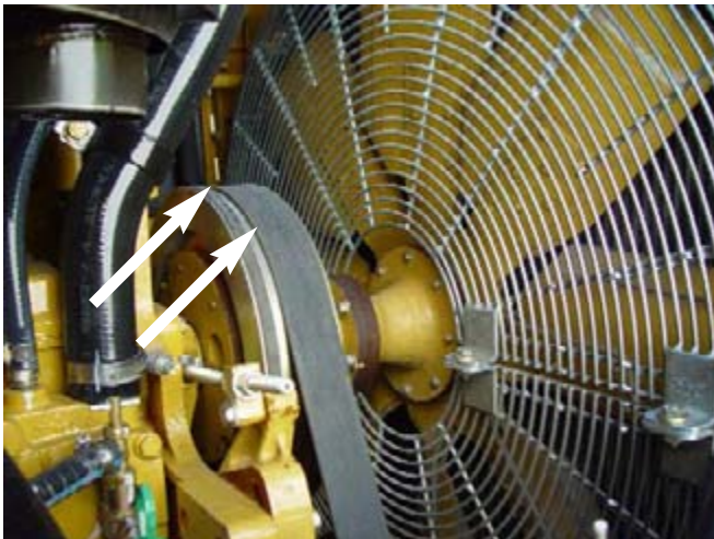
Fig. 75: When fan belts and pulleys are in good condition belts extend beyond the edge of the pulley.
