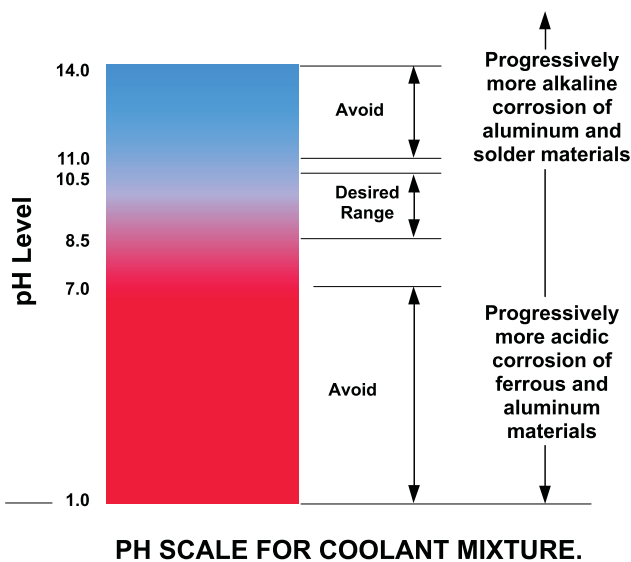
Fig. 52: pH scale for coolant mixture.
