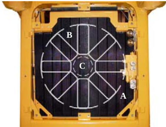
Fig. 70: Critical locations of the radiator core.
