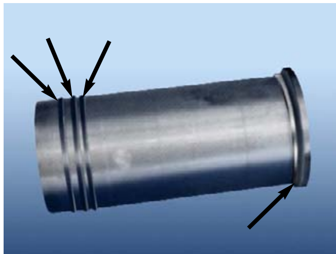
Fig. 80: Filler band and O-ring seals on cylinder liner.
