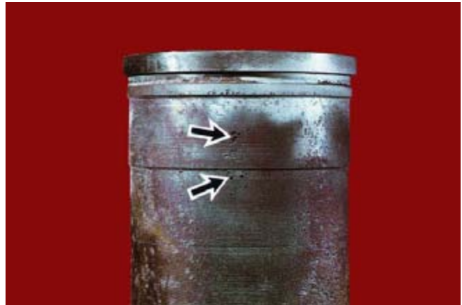
Fig. 45: Example of cylinder wall cavitation-erosion.
