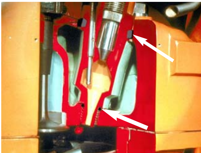
Fig. 79: O-ring seals and gasket on precombustion chamber.
