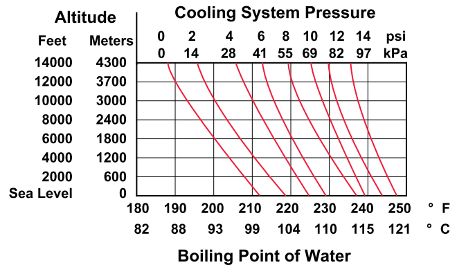
Fig 5: Pressure/temperature chart.
