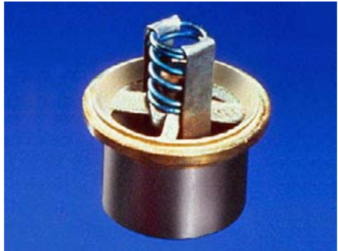
Fig. 67: Bonnet-type water temperature regulator.
