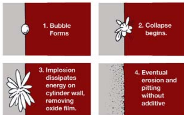
Fig. 46: Progression of cavitation and pitting on cylinder wall.
