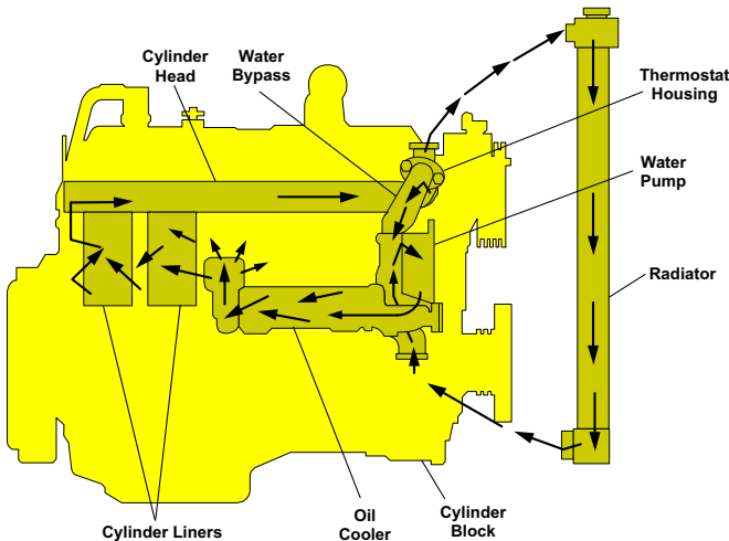
Fig 2: Typical Cooling System.
