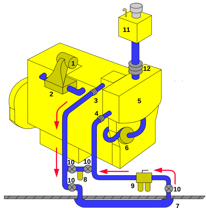
Fig. 3: Schematic of typical heat exchanger cooling system.
